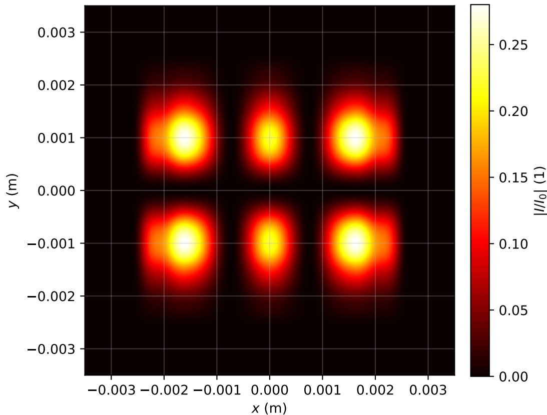
Intensity profile I(x, y, z = 3.582)/I_0 , P_{in}=1.0P_{cr} , artificial time
